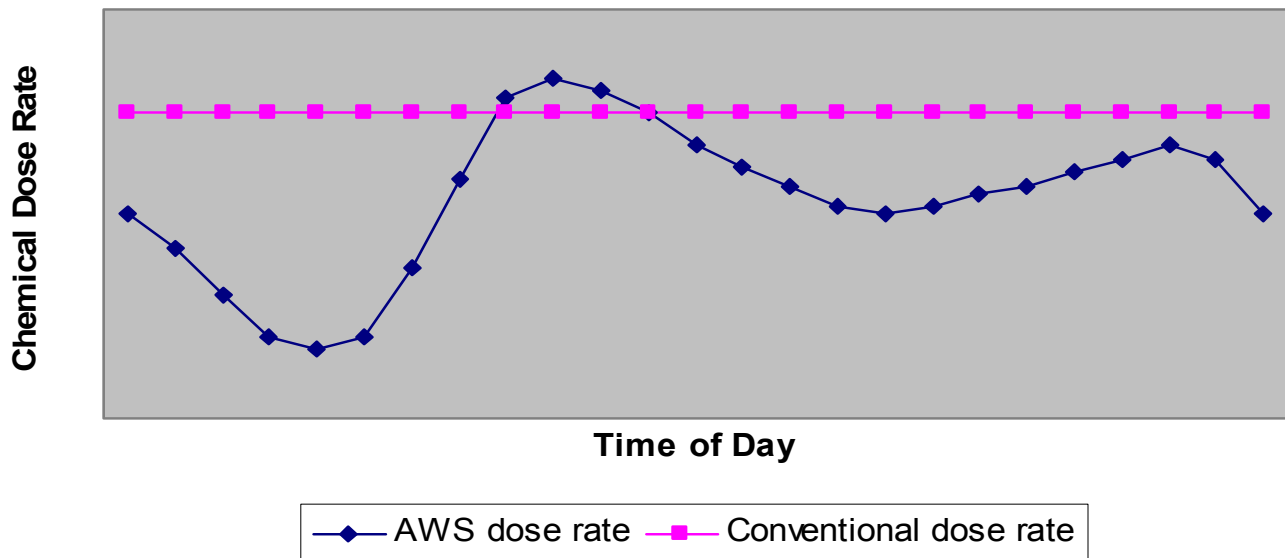
Comparison of Typical Chemical Dose Rates for AWS System vs. Conventional System
